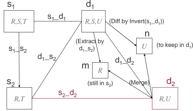
Figure 2: Propagating changes by the view s_{1-s_2}
